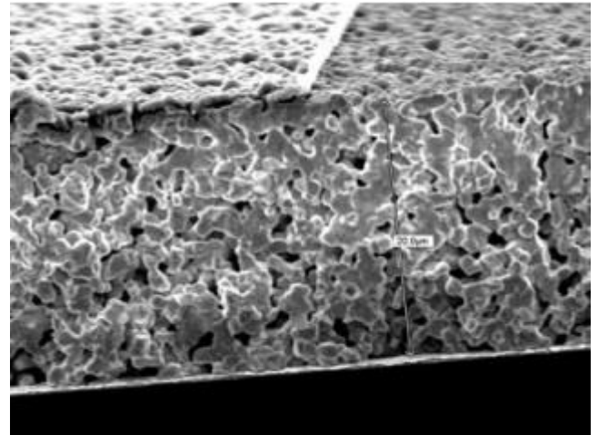
SEM picture of TF2100 microstructure
