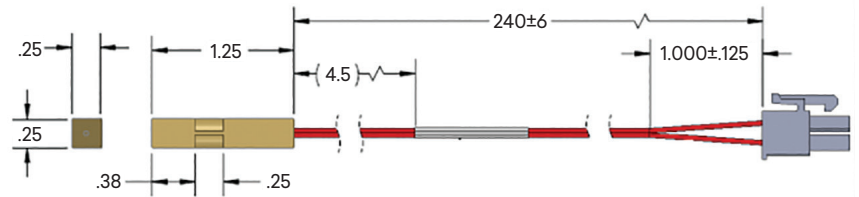
FIGURE 2: SENSOR IN MACHINED BRASS HOUSING
