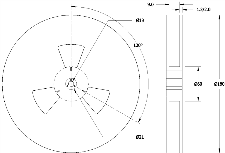
Reel Drawing
