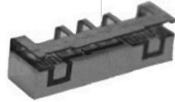
Part Dimensions: 11.7 × 3.2 × 3.7 mm • 0.35 g Materials: Ag plated ceramic block with fused-tin plated brass shield
