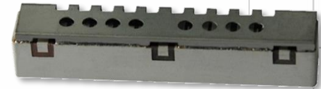
Part Dimensions: 63.0 × 11.4 × 10.6 mm • 21.0 g Materials: Ag plated ceramic block with tin plated brass shield
