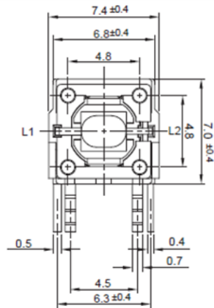
Figure 3 – 228FDS, Standard Though Hole, Side Actuation
