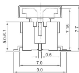
Figure 3 – 228FDS, Standard Though Hole, Side Actuation
