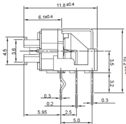
Figure 3 – 228FDS, Standard Though Hole, Side Actuation
