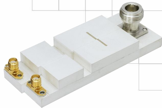
Part Dimensions: <100 x <40 x <14.5 mm • <150 g Materials: Ag plated ceramic block
