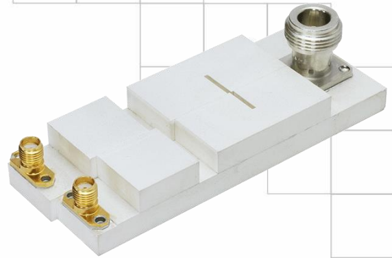
Part Dimensions: 94 x 35 x 14.5 mm • <195 g Materials: Ag plated ceramic block
