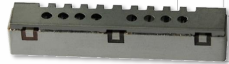
Part Dimensions: 61.6 × 11.4 × 10.9 mm • 22.1 g Materials: Ag plated ceramic block with tin plated brass shield
